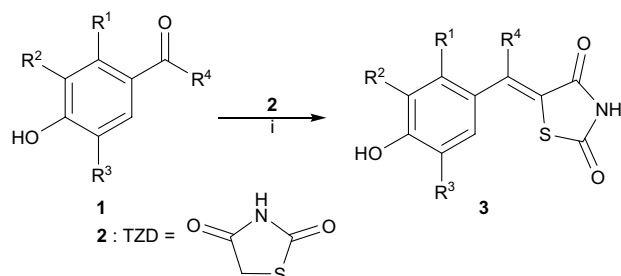
Scheme 1. Reagents and reaction conditions: (i) method A: piperidine (cat.), EtOH, reflux; method B: NH 4 OAc, toluene, reflux.
