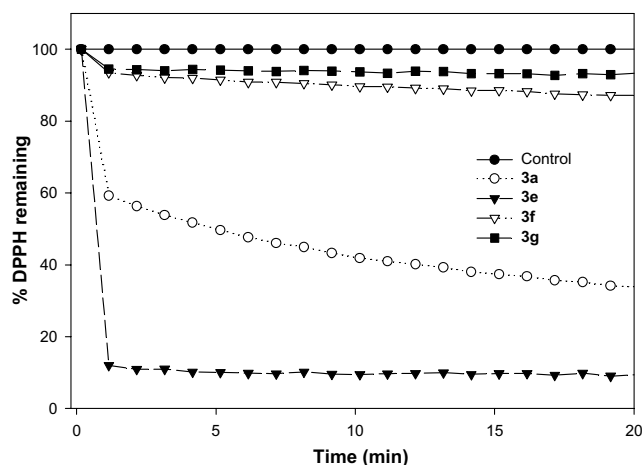
Figure 4. Effects of 3a , 3e , 3f , and 3g on radical DPPH scavenging. Compounds 3a , 3e , 3f , and 3g (100 \mu M) were incubated with 100 \mu M of DPPH in methanol at room temperature for 20 min. The absorbance at 517 nm of each compound solution was measured. The antiradical activity was expressed by the remaining DPPH percentage.
