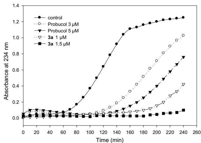
Figure 1. Effect of 3a on \text{Cu}^{2+} -mediated LDL oxidation. LDL (100 \mu\text{g} protein/mL) was incubated with 5 \mu\text{M} of \text{CuSO}_4 in the presence or absence of antioxidant, 3a . Conjugated diene formation was measured by determining the absorbance at 234 nm every 10 min for 4 h. Probucol was used as a reference antioxidant.
